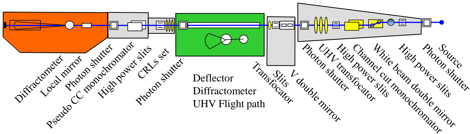
CXS – EH2 in operation
